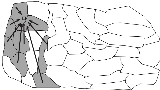
FIGURE 6 Example of focal zone seed transfer system (a) without and (b) with assisted migration. In (a), the genetic suitability area consists of all zones that are climatically similar to the focal zone (i.e., the zone containing the planting site); in (b), the genetic suitability area shifts toward warmer zones south of the focal zone.
