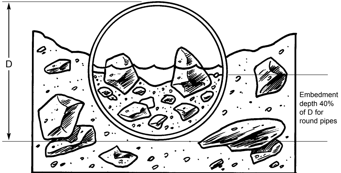
Culvert/streambed cross-section
