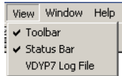
Figure 2-20: View Menu
