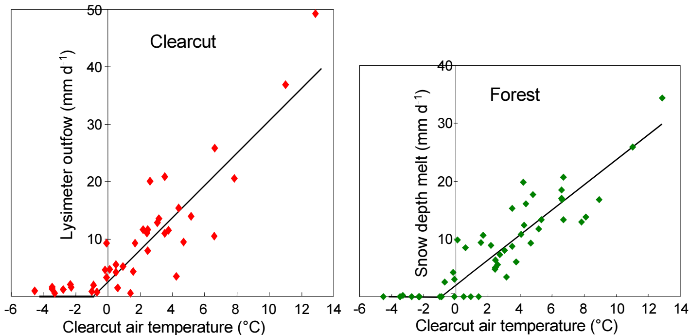
Figure 3. Data for 1999 melt season used to determine the melt factors for the air temperature index method in the clearcut and forest. The lines indicate the equations given in the text.
