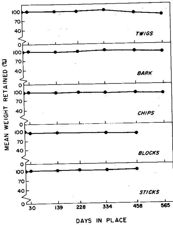
Figure 9. Weight loss in five fine wood substrates of Douglas-fir placed on the forest floor and in Mack Creek on the H. J. Andrews Forest. Each point is the mean of three samples.
