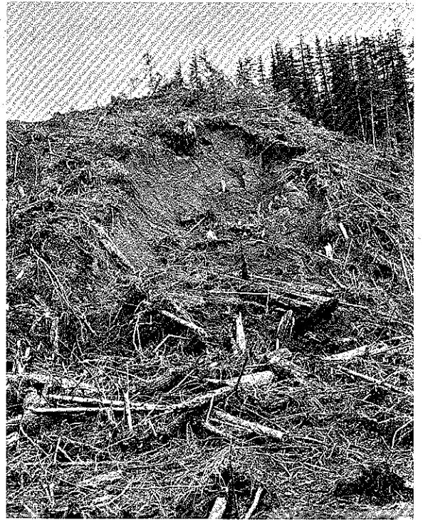
Figure 4-b. Massive earthflow in a recently logged area on the west flank of the Cascades. Depth of soil not available, but failure occurred in relatively deeply weathered pyroclastic materials.
