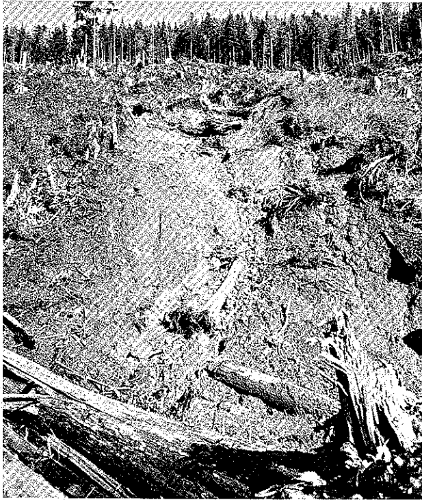
Figure 4. Examples of natural slumps and earthflows. a) Massive slump and earthflow in a weathered till bank near Hollis, Prince of Wales Island, Alaska. Depth of weathering approximately 4 feet. Slope approximately 15^\circ (34 percent grade).
