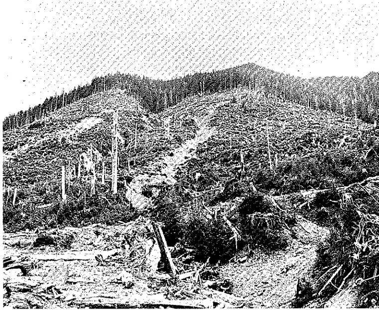
Figure 2-a. Debris avalanche, debris flow combination on a recently logged, till-covered slope. Failure occurred during a period of high intensity rainfall in a zone of concentrated subsurface drainage. The sliding material was weathered till less than 1.0 meter thick overlying compacted unweathered till. The slope angle is about 34^{\circ} (75 percent grade). Note scouring of the avalanche path below spoon-shaped zone of initial failure and flow development at slope base.
