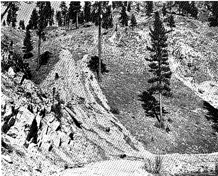
Figure 2-b. Debris avalanches along the South Fork of the Salmon River, Idaho. These failures occurred in a shallow granitic soil following saturation during a high intensity rainstorm. The soil is a lithosol less than 0.3 meter thick. The slope is in excess of 31^{\circ} (70 percent grade).
