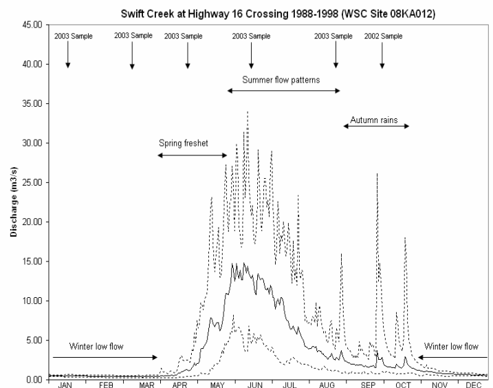
Figure 2. Lowest (bottom line), average (middle line) and maximum (upper line) daily flows observed in Swift Creek over the period 1988-1998.
