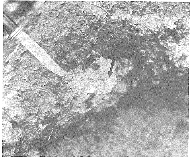
Figure 3.—Primary root showing resin-encrusted lesion common on many roots of trees infected with A. mellea .
